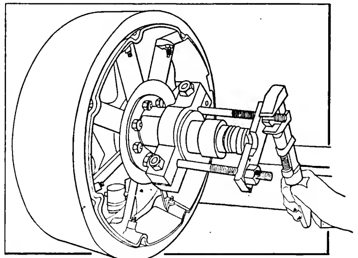
Fig. 4—Showing the method and tools used in compressing the clutch spring
